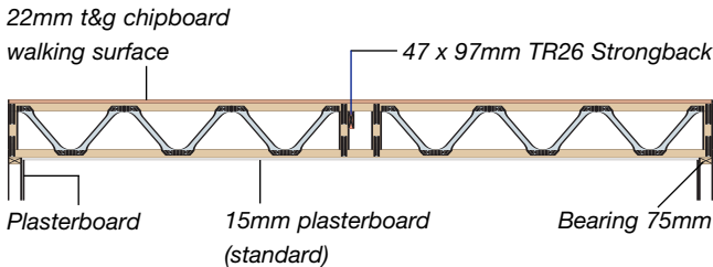
Separating floor construction: 60 minutes fire resistance
