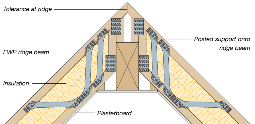
Ridge detail
