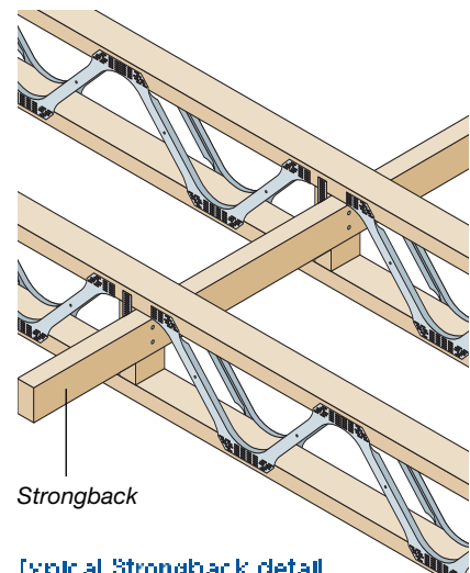
Typical Strongback detail
