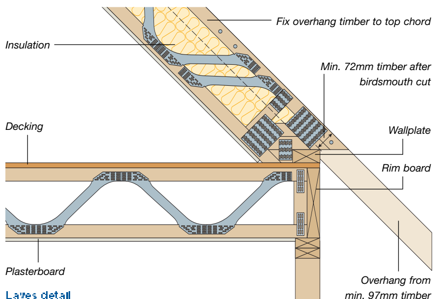
Eaves detail
