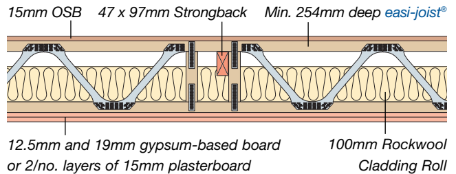
Separating floor construction: 60 minutes fire resistance
