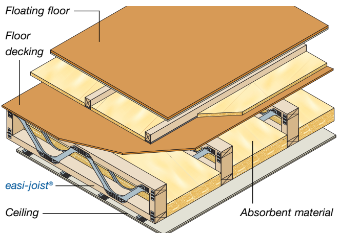
Separating floor construction (Robust Detail E-FT-3)
