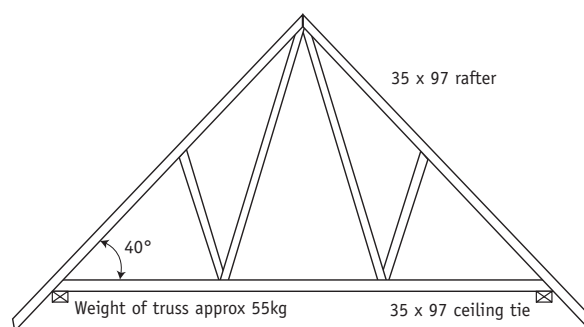
Fig. 1 Typical 8 metre span conventional trussed rafter
