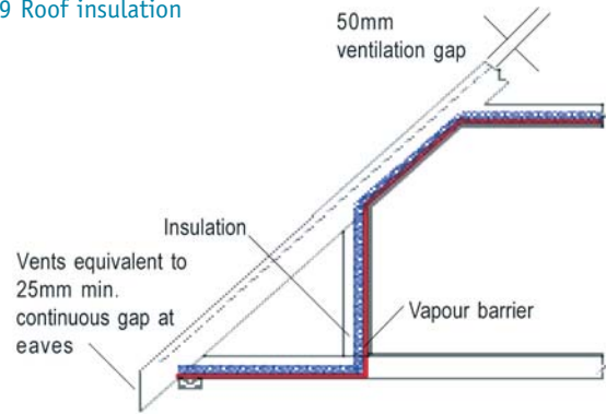
Fig. 9 Roof insulation - alternative arrangement
