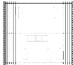
Unsuitable layout - very difficult to provide 'RiR' trusses to support this roof since windows and stairs all overlap
